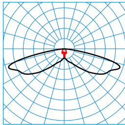
Publisca P2-SB3L/1000-730 2G1S ETDD (CLO initial value) TX300973 ■ C0 - C180 ■ C90 - C270 DIN 5040: A30 UTE: 1,00 l DLOR: 100 % ULOR: 0 % CEN Flux Code: 31 65 93 100 100
