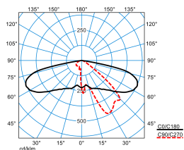
Publisca P2-AB2L/2000-730 3G1S ETDD (CLO initial value)
