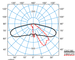
Publisca P2-AB2L/2000-730 3G1S ETDD (CLO end value)
