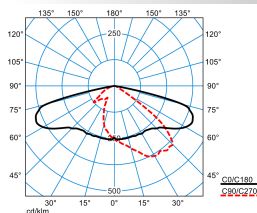
LIQ 70N-AB7L-LRA/10/12/135-730 12G1 ETDD(CLO end value) TX278275
