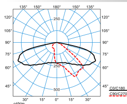
LIQ 50N-AB2L-SLR2/6800-727 6G1 ET (CLO initial value)
