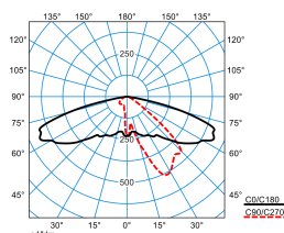
Publisca P1W-AB2L/3800-730 6G1S ETDD (CLO end value)
