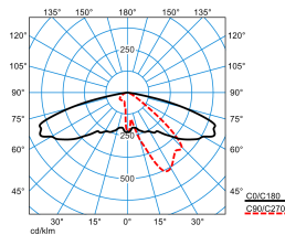
Publisca P1W-AB2L/3800-730 6G1S ETDD (CLO initial value)
