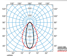
ELINE PN55-120 ML 830 L225 0 50
