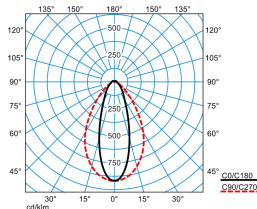
ELINE PN55-120 ML 830 L225 4 50
