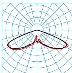
Publisca P1-RB6L-LRA/2600-740 3G1S ET (CLO initial value) TX300609 ■ C0 - C180 ■ C90 - C270 DIN 5040: A20 UTE: 1,00 J DLOR: 100 % ULOR: 0 % CEN Flux Code: 20 57 98 100 100
