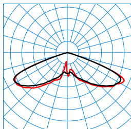
Publisca P1-RB6L-LRA/2600-740 3G1S TX047672 ■ C0 - C180 ■ C90 - C270 DIN 5040: A20 UTE: 1,00 J DLOR: 100 % ULOR: 0 % CEN Flux Code: 20 57 98 100 100
