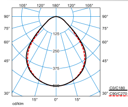
Opendo D2-L PW19 42-840 ETDD +LLWM 01 TX277490
