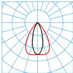
ELINE LVN80 865 L225 1 50
