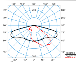
LIQ 70N-AB7L-LR/75/82/91-727 10G1 ET(CLO initial value)
