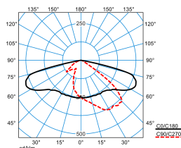
LIQ 70N-AB7L-LR/75/82/91-727 10G1 ET(CLO end value)
