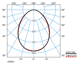
SFlow C1-L MRWD LED3200-830 ETDD 01 TX721353
