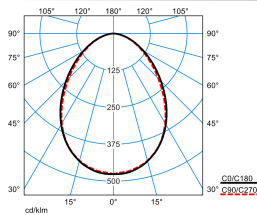
SFlow C1-L MRWD LED3200-830 ETDD 01 TX771460
