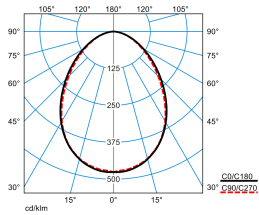
SFlow C1-L MRWD LED3200-830 ETDD 01 TX771460
