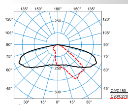
LIQ 50N-AB2L-SLR2/6800-727 6G1 ET (CLO initial value)
