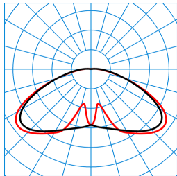
Publisca P1W-RBT-LRA/1500-740 2G1S TX053580 ■ C0 - C180 ■ C90 - C270 DIN 5040: A20 UTE: 0.97 l + 0.03 T DLOR: 97 % ULOR: 3 % CEN Flux Code: 26 63 91 97 100 4 16 28 3
