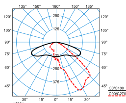
Publisca P2-AB2L-LR/3500-740 4G1S ET (CLO initial value) TX301227 DIN 5040: A30 UTE: 1,00 G DLOR: 100 % ULOR: 0 % CEN Flux Code: 35 73 97 100 100
