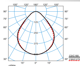
Opendo M39 PW19 42-8TW ETDD8 (DWW)
