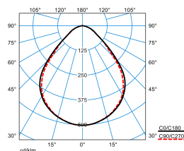
Opendo M39 PW19 42-8TW ETDD8 (DCW)
