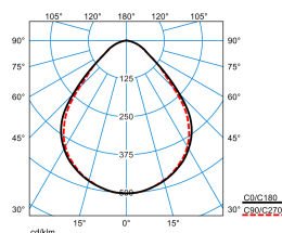
Opendo M39 PW19 42-8TW ETDD8 (DSU)
