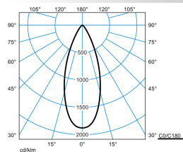
Altigo G2 120 RB17L/3800-830 1G1P + VE IP66 24V DC 250W
