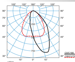
ELINE HE LAN60 827 L225 2 20
