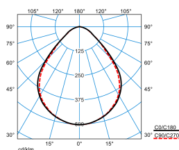
Opendo D2-L PW19 47-8TW ETBLE +CAS 03 (DSU)
