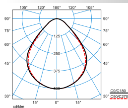
Opendo D2-L PW19 47-8TW ETBLE +CAS 03 (DWW)
