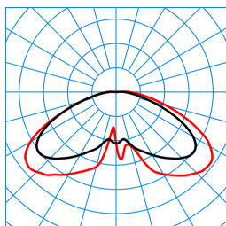
Publisca P1W-RBT-LR/2600-730 3G1S ET (CLO initial value) TX301736 ■ C0 - C180 ■ C90 - C270 DIN 5040: A20 UTE: 0.99 l + 0.01 T DLOR: 99 % ULOR: 1 % CEN Flux Code: 26 63 91 99 100 0 0 0 1
