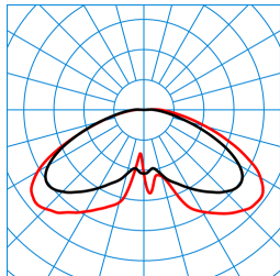
Publisca P1W-RBT-LR/2600-730 3G1S TX053573 ■ C0 - C180 ■ C90 - C270 DIN 5040: A20 UTE: 0.99 l + 0.01 T DLOR: 99 % ULOR: 1 % CEN Flux Code: 26 63 91 99 100 0 0 0 1
