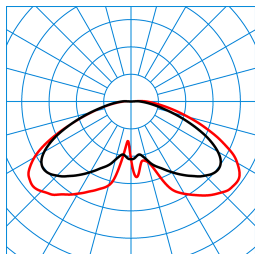
Publisca P1W-RBT-LR/2600-730 3G1S ET (CLO end value) TX300608 ■ C0 - C180 ■ C90 - C270 DIN 5040: A20 UTE: 0.99 l + 0.01 T DLOR: 99 % ULOR: 1 % CEN Flux Code: 26 63 91 99 100 0 0 0 1
