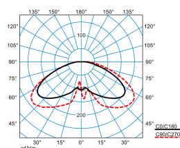
Publisca P1W-RBT-LR/2600-730 3G1S
