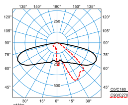
Publisca P2-AB2L/2200-730 3G1S ETDD (CLO end value) TX301884 DIN 5040: A30 UTE: 1,00 l DLOR: 100 % ULOR: 0 % CEN Flux Code: 34 71 96 100 100
