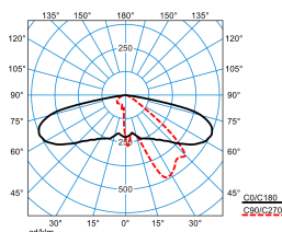
Publisca P2-AB2L/2200-730 3G1S ETDD (CLO initial value) TX300451 DIN 5040: A30 UTE: 1,00 l DLOR: 100 % ULOR: 0 % CEN Flux Code: 34 71 96 100 100
