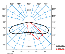
LIQ 50N-AB2L-LRA/1500-730 2G1 ETDD (CLO initial value) TX778229
