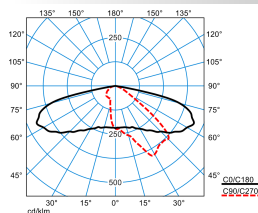
LIQ 50N-AB2L-LRA/1500-730 2G1 ETDD (CLO end value) TX778224
