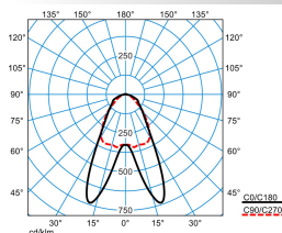
ELINE HE LDAN60-160 ML 830 L225 0 20
