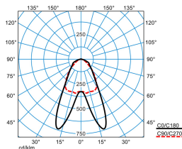
ELINE HE LDAN60-160 ML 830 L225 2 20
