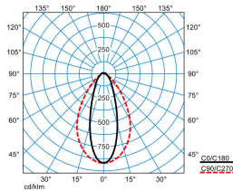
ELINE HE PN60-150 ML 830 L225 2 50
