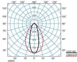
ELINE HE PN60-150 ML 830 L225 4 50
