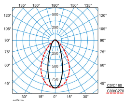
ELINE HE PN60-150 ML 830 L225 0 50
