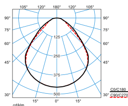
ValineoG5 IP M73 PW19 38-50/4ML-8MC ETDD (stage 2)
