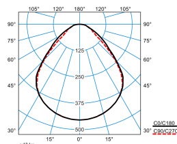
ValineoG5 IP M73 PW19 38-50/4ML-8MC ETDD (stage 6)
