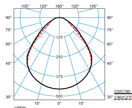
ValineoG5 IP M73 PW19 38-50/4ML-8MC ETDD (stage 7)
