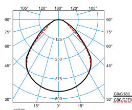
ValineoG5 IP M73 PW19 38-50/4ML-8MC ETDD (stage 3)
