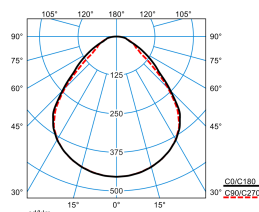
ValineoG5 IP M73 PW19 38-50/4ML-8MC ETDD (stage 8)
