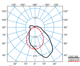
TugraHE 6 PAW 23-38/16ML-840 ET PC 23 (stage 8)
