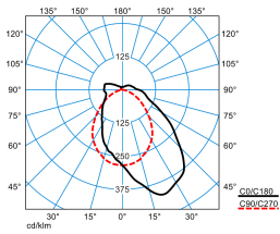
TugraHE 6 PAW 23-38/16ML-840 ET PC 23 (stage 4)
