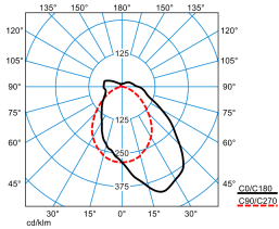
TugraHE 6 PAW 23-38/16ML-840 ET PC 23 (stage 5)
