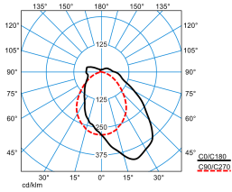
TugraHE 6 PAW 23-38/16ML-840 ET PC 23 (stage 3)
