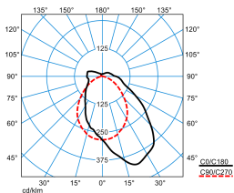
TugraHE 6 PAW 23-38/16ML-840 ET PC 23 (stage 7)
