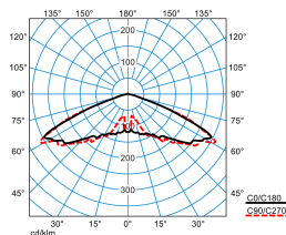
Publisca P1W-RB6L/1500-740 2G1S ETDD (CLO initial value) TX301828
