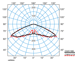
Publisca P1W-RB6L/1500-740 2G1S ETDD (CLO end value) TX301118
