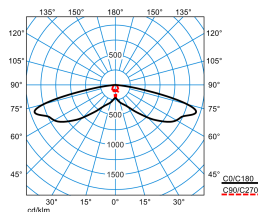
Publisca P2-SB3L/800-730 2G1S ETDD (CLO initial value) TX300293 DIN 5040: A30 UTE: 1,00 l DLOR: 100 % ULOR: 0 % CEN Flux Code: 31 65 93 100 100
