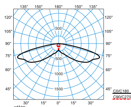
Publisca P2-SB3L/800-730 2G1S ETDD (CLO end value) TX300629 DIN 5040: A30 UTE: 1,00 l DLOR: 100 % ULOR: 0 % CEN Flux Code: 31 65 93 100 100
