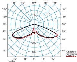
Publisca P1-RB6L-LR/2600-730 3G1S ET (CLO end value) TX301073 DIN 5040: A20 UTE: 1,00 J DLOR: 100 % ULOR: 0 % CEN Flux Code: 20 57 98 100 100
