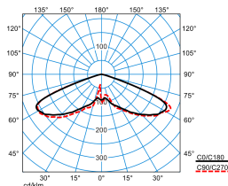
Publisca P1-RB6L-LR/2600-730 3G1S ET (CLO initial value) TX301714 DIN 5040: A20 UTE: 1,00 J DLOR: 100 % ULOR: 0 % CEN Flux Code: 20 57 98 100 100
