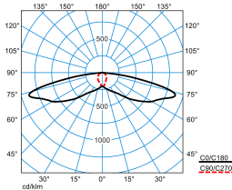
LIQ 50N-SB3L-LR/1500-730 2G1 ET (CLO end value) TX779663
