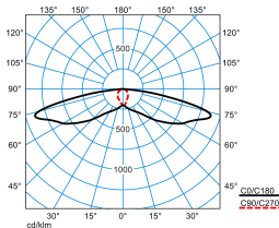
LIQ 50N-SB3L-LR/1500-730 2G1 ET (CLO initial value) TX779670
