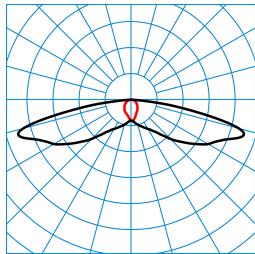
LIQ 50N-SB3L-LR/1650-730 2G1 ET (CLO initial value) TX777017 ■ C0 - C180 ■ C90 - C270 DIN 5040: A30 UTE: 1,00 l DLOR: 100 % ULOR: 0 % CEN Flux Code: 31 64 92 100 100
