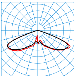
Publisca P2-RB6L/2200-740 3G1S ETDD (CLO initial value) TX301654 ■ C0 - C180 ■ C90 - C270 DIN 5040: A20 UTE: 1,00 J DLOR: 100 % ULOR: 0 % CEN Flux Code: 20 57 98 100 100
