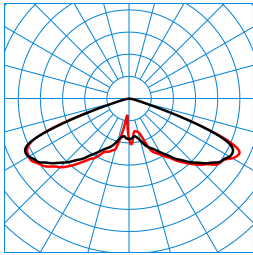
Publisca P2-RB6L/2200-740 3G1S ETDD (CLO end value) TX301781 ■ C0 - C180 ■ C90 - C270 DIN 5040: A20 UTE: 1,00 J DLOR: 100 % ULOR: 0 % CEN Flux Code: 20 57 98 100 100
