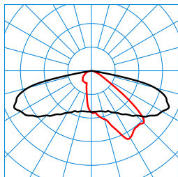
LIQ 50N-AB2L-LR/2900-722 4G1 ET (CLO initial value) TX777687 ■ C0 - C180 ■ C90 - C270 DIN 5040: A30 UTE: 1,00 G DLOR: 100 % ULOR: 0 % CEN Flux Code: 34 71 96 100 100 0 0 0 0
