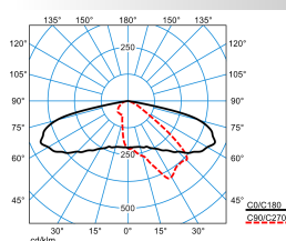
LIQ 50N-AB2L-LR/220/260/320-727 4G1 ET (CLO initial value)
