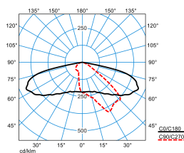
LIQ 50N-AB2L-LR/220/260/320-727 4G1 ET (CLO end value)
