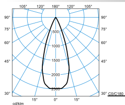
Linell 3PID5 LW19-FL-05 11-930 ETDD 05
