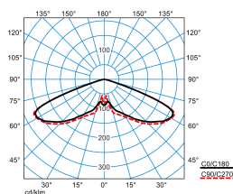
Publisca P2-RB6L/2900-740 4G1S ETDD (CLO initial value)
