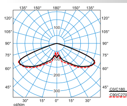
Publisca P2-RB6L/2900-740 4G1S
