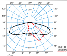
LIQ 50N-AB2L-LR/135/165/200-727 2G1 ET (CLO initial value)
