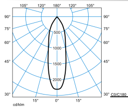
TokoP RF-MF 40-BC M51 ETBLE 05
