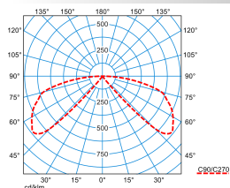
Skeo Q-B1-15-2 AM8R/500-740 1G1P ET TX779592
