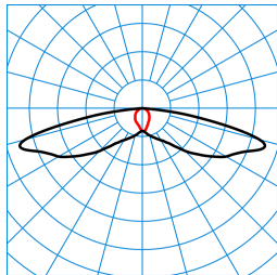
LIQ 50N-SB3L-SLR2/2200-740 2G1 ET (CLO end value) TX779474
