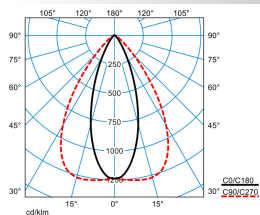
ELINE LVN100 840 L150 1 50
