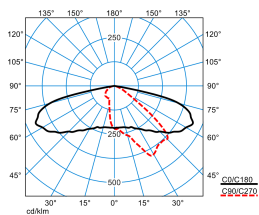
LIQ 50N-AB2L-LRA/2200-740 4G1 ETDD (CLO end value)
