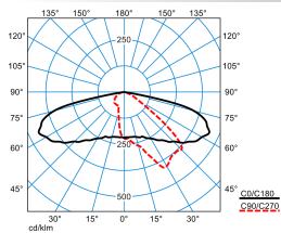
LIQ 50N-AB2L-LRA/2200-740 4G1 ETDD (CLO initial value)
