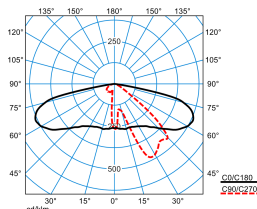
Publisca P1-AB2L/1000-730 2G1S ETDD (CLO end value) TX300765 DIN 5040: A30 UTE: 1,00 G DLOR: 100 % ULOR: 0 % CEN Flux Code: 34 70 96 100 100
