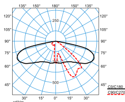
Publisca P1-AB2L/1000-730 2G1S ETDD (CLO initial value) TX301095 DIN 5040: A30 UTE: 1,00 G DLOR: 100 % ULOR: 0 % CEN Flux Code: 34 70 96 100 100
