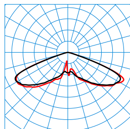
Publisca P2-RB6L/2600-740 3G1S ETDD (CLO end value) TX300521 ■ C0 - C180 ■ C90 - C270 DIN 5040: A20 UTE: 1,00 J DLOR: 100 % ULOR: 0 % CEN Flux Code: 20 57 98 100 100
