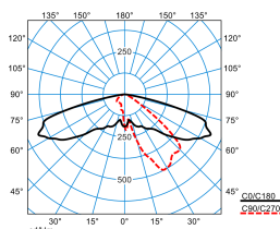
Publisca P1W-AB2L-LR/3200-740 4G1S
