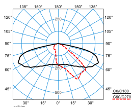
LIQ 50N-AB2L-LRA/2400-730 4G1 ETDD (CLO initial value) TX778670
