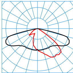
LIQ 70N-AB7L-LR/10000-722 12G1 ET (CLO initial value) TX778178 ■ C0 - C180 ■ C90 - C270 DIN 5040: A30 UTE: 1,00 E DLOR: 100 % ULOR: 0 % CEN Flux Code: 39 76 98 100 100
