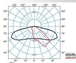
LIQ 50N-AB2L-LR-SLR2/4200-730 4G1 ET (CLO initial value)
