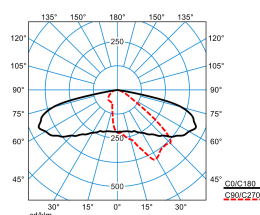
LIQ 50N-AB2L-LR-SLR2/4200-730 4G1 ET (CLO end value)
