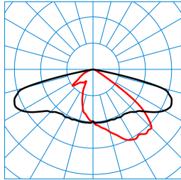
LIQ 70N-AB7L-SLR2/16000-730 12G1 ET (CLO end value) TX775491
