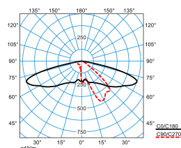
Publisca P1W-AB2L-LR/2200-730 3G1S
