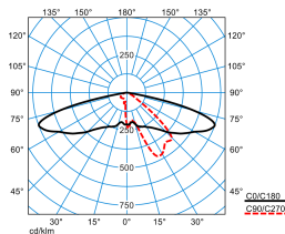
Publisca P1W-AB2L-LR/2200-730 3G1S
