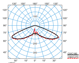
Publisca P1W-RB6L-LRA/2200-740 3G1S
